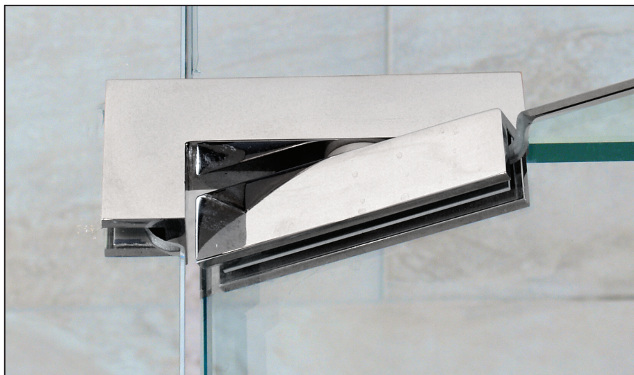
C.G.M. glass to transom glass to hinge
